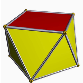
Square Antiprism
